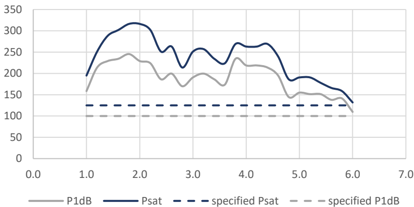
Typical performance
